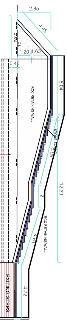
SECTION X-X
